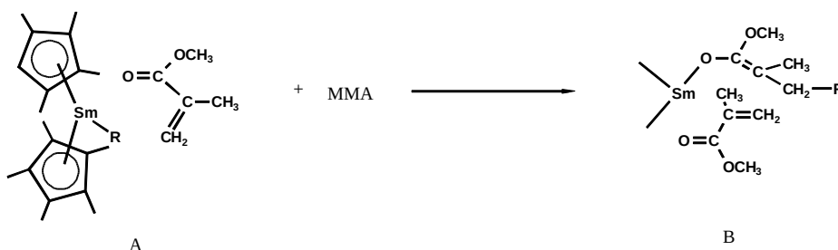
Scheme 1.8 : Initiation of MMA with Lanthanide III complexes
