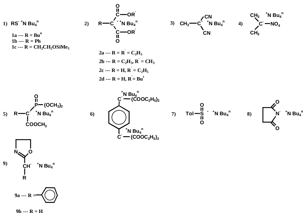
Scheme 1.9 : Metal-free carbanions for alkyl(meth)acrylate polymerization
