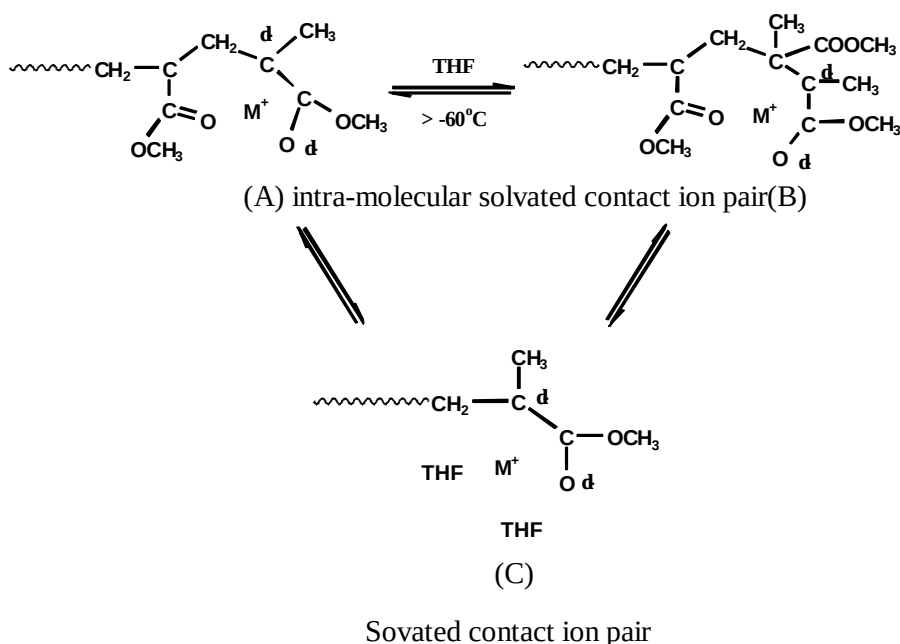
Scheme 1.3: Propagation via contact ion pairs in MMA polymerization
