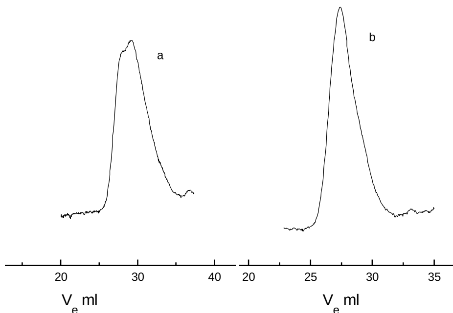
Fig: 7.4: GPC elugrams of polyacrylates synthesized using tetrabutylammonium diethylphenylmalonate, 1a , as initiated in THF at 30 °C. a) poly( n -butylacrylate), M_{n,SEC} = 23,700 , M_w/M_n = 2.73 and b) poly( tert -butylacrylate), M_{n,SEC} = 38,300 , M_w/M_n = 1.69 .
