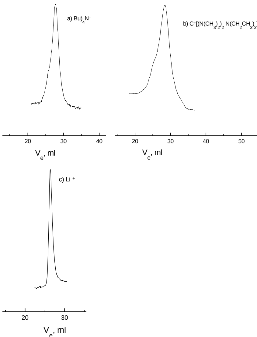
Fig 7.7: GPC elugrams of Polymethylmethacrylate samples synthesized in presence of different counteranion in THF at -40\text{ }^\circ\text{C} . The polymerization of MMA was initiated using 1,1'-diphenylhexyl anion with a) in presence of tetrabutylammonium counterion, b) in presence of tetramethyldiethylguanidinium counterion and c) in presence of lithium counterion.
