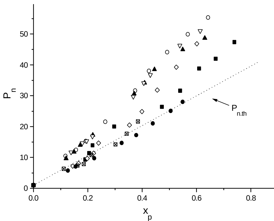
Fig. 5.13: Dependence of number average degree of polymerization, P_n , on conversion x_p . r = [\text{LiClO}_4]_0/[\text{DPHLi}]_0 ; (■) r = 0 , (○) r = 0.3 , (▲) r = 0.6 , (Δ) r = 1 , (◇) r = 3 , (⊠) r = 5 , and (●) r = 10 .
