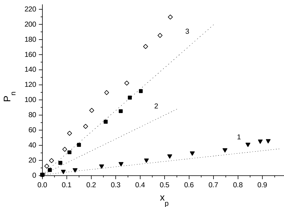
Fig. 4.3: Dependence of degree of polymerization, P_n with conversion, x_p of MMA polymerization using TMEDA chelated \text{Li}^+ counterion at -20^\circ\text{C} in THF. [\text{M}]_0=0.23 \text{ mol/l} , [\text{I}]_0 ; 1) 5.9 \cdot 10^{-3} , 2) 1.4 \cdot 10^{-3} and 3) 0.8 \cdot 10^{-3} all in mol
