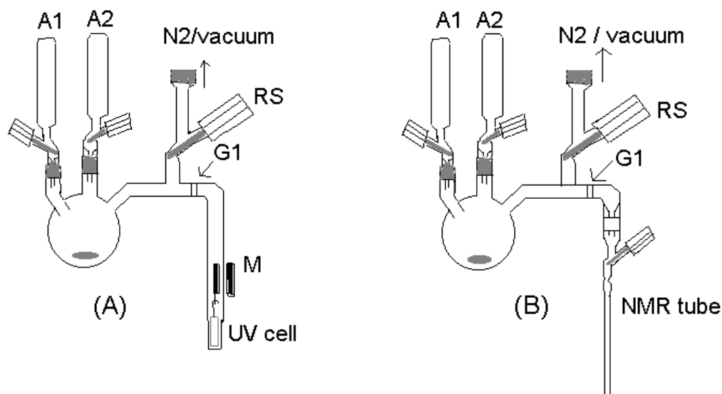
Fig. 6.1: Apparatus used for the UV and NMR analysis of initiator solution. A1, A2- ampoules THF (or THF- d_8 ) and precursor initiator, RS rota-flow stop-cocks, G1- coarse frit, M- magnet for holding the UV cell spacer.
