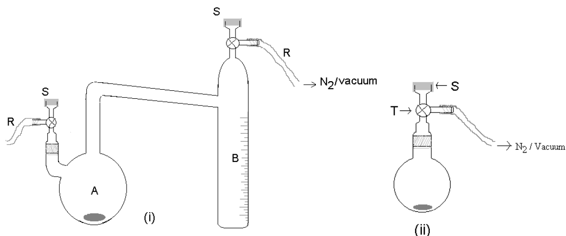
Fig. 3.1: Distillation apparatus (i) and batch polymerization reactor (ii) for anionic polymerization of alkyl(meth)acrylate; (S) rubber septum, (R) natural rubber tube for taking N_2 /vacuum from manifold, and (T) three-way stop-cock.
