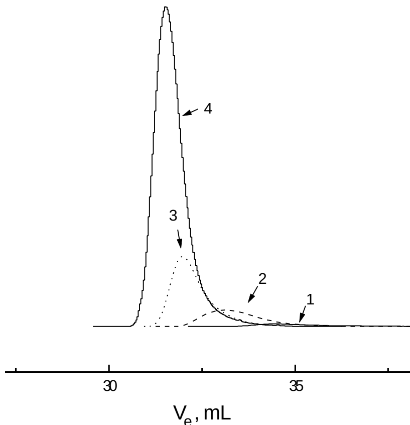
Fig. 5.6: SEC traces of PMMA samples at various time of polymerization in presence of \text{LiClO}_4 in Toluene/THF (9:1 v/v) at -78\text{ }^\circ\text{C} ; 1. after 10 mins., 2. after 40 mins., 3. after 80 mins., and 4. after 120 mins.
