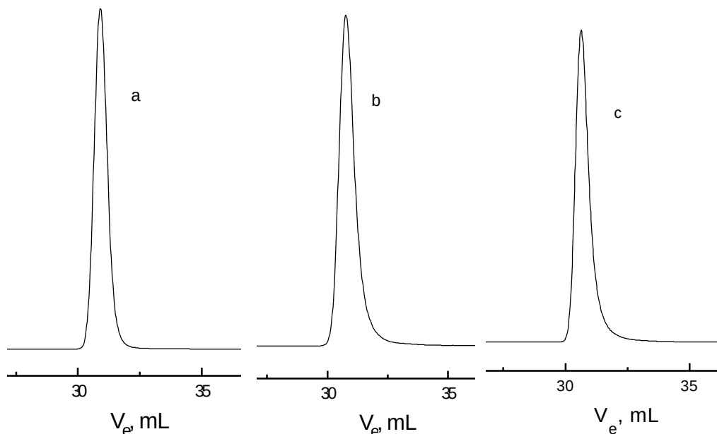
Fig. 5.1: SEC traces showing the effect of \text{LiClO}_4 addition on anionic
