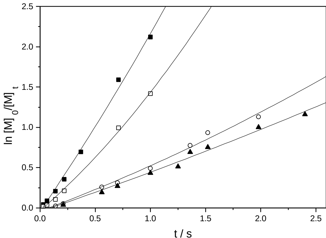
Fig. 6.2: First-order time-conversion plots of the anionic polymerization of MMA using \text{Ph}_3\text{C}^+\text{P}^-\text{Ph}_4 counterion at various initiator concentrations in THF at 0 °C. [\text{M}]_0 = 0.2 \text{ mol/L} , [\text{I}]_0 : (■) 9.95 \cdot 10^{-3} , (□) 5.3 \cdot 10^{-3} , (○) 2.37 \cdot 10^{-3} , and (▲) 1.42 \cdot 10^{-3} all in mol/L.
