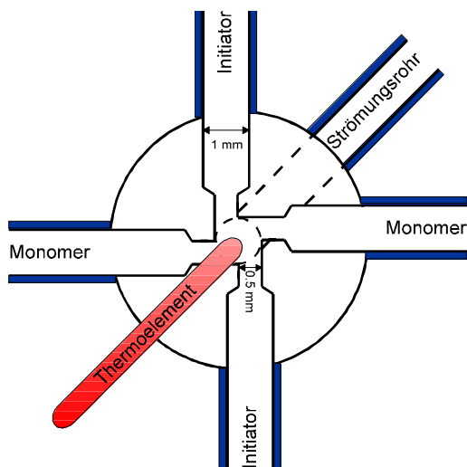
Fig. 3.4: Four-way mixing jet of the flow-tube reactor.
