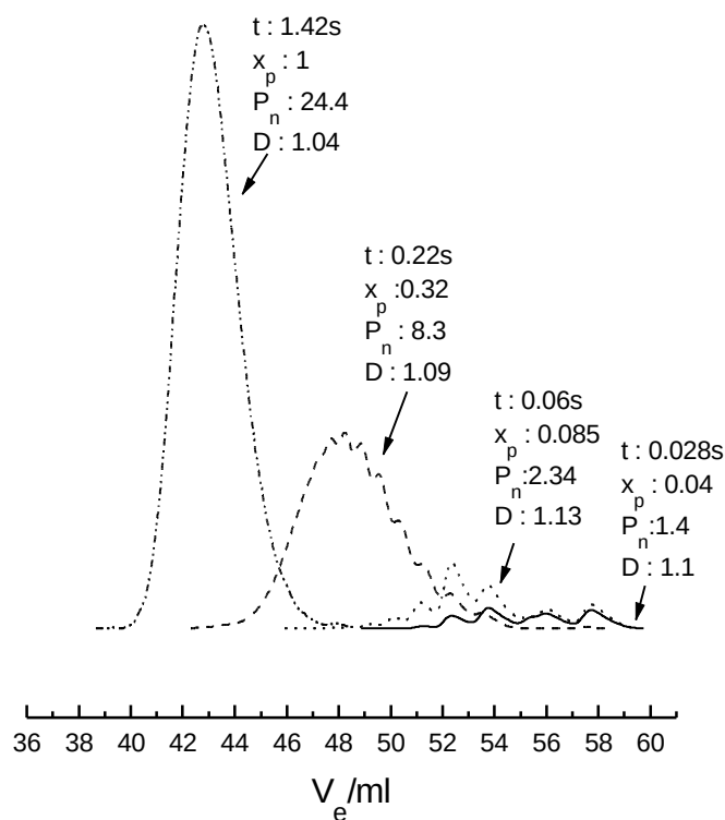
Fig. 6.4: SEC eluograms at different times during the polymerization of MMA using \text{PPh}_4 counterion in THF. [\text{M}]_0 = 0.2 \text{ mol/L} , [\text{I}]_0 = 9.95 \cdot 10^{-3} \text{ mol/L} (run No. 4 in Table 6.4).
