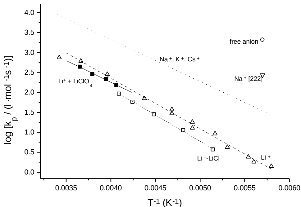
Fig. 5.16: Arrhenius plot of the propagation rate constants, k_p in the anionic polymerization of MMA in THF for Li counterion with \text{LiClO}_4 ligand and the reported rate constants for other counterion and solvent (Aggregation was not taken into account).
