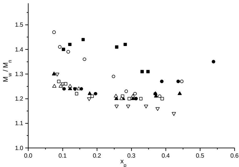
Fig. 4.7: Dependence of MWD on conversion in presence of various amount of TMEDA; r = (\bullet), 0.3 (\blacksquare), 0.7 (O), 1 (\blacktriangle), 1.5 (\nabla), 3.5 (\square), \text{ and } 7 (\Delta) .
