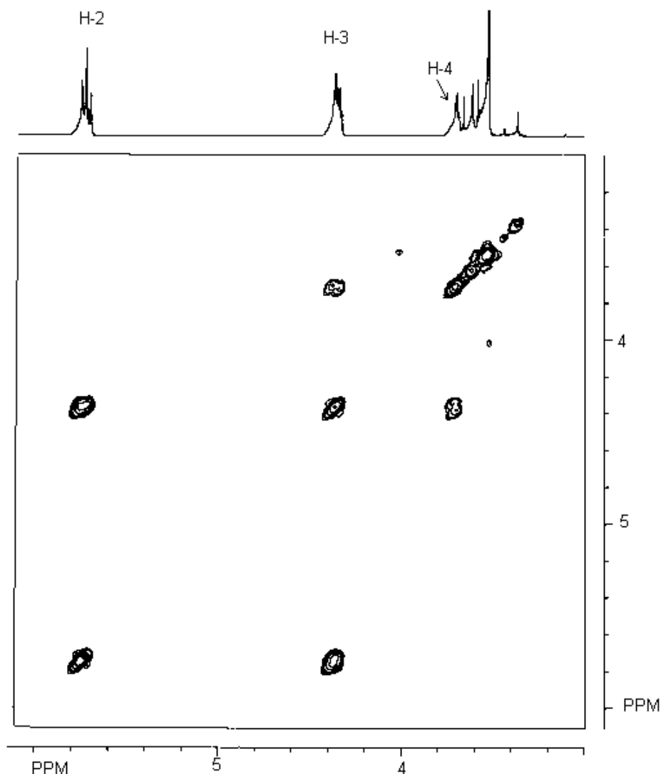
Fig. 16.15: 2D ^1\text{H} , ^1\text{H} - COSY spectrum of 4 showing a long-range coupling of the cyclohexadienyl ring proton
