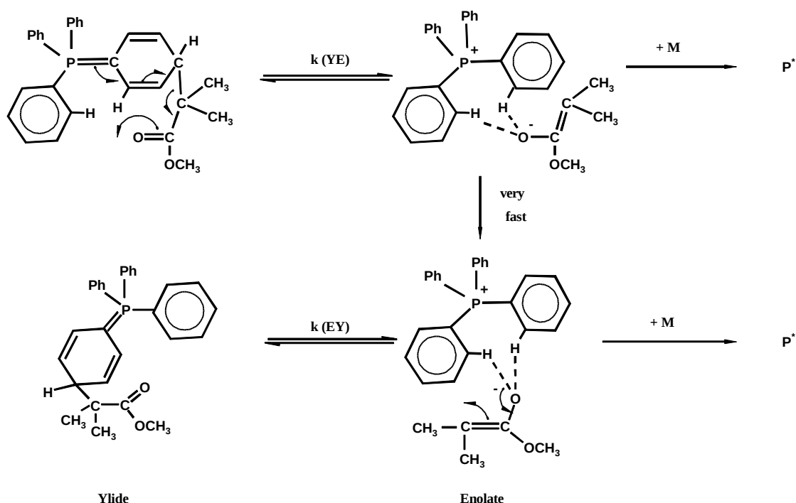
Scheme 6.6: Exchange of ylide MIB group via ion pair
