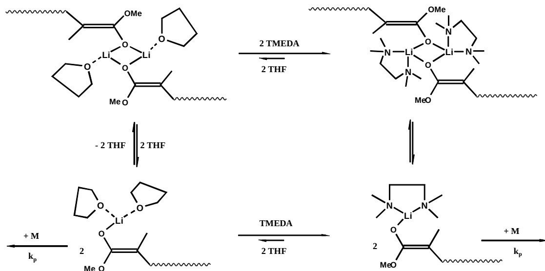
Scheme 1: Chelation and aggregation of PMMA-Li
