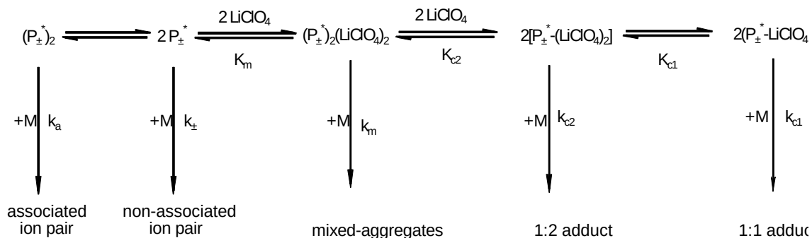
Scheme 5.1: Formation of adduct in the presence of LiClO 4 in the anionic polymerization of MMA in THF
