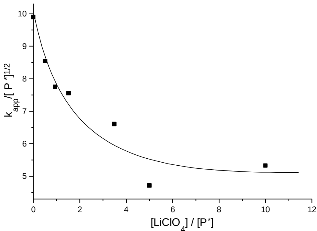
Fig. 5.14: Effect of LiClO_4 concentration on the rate constant, k_p , of MMA polymerization in THF at -20^\circ C .
