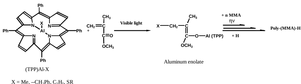
Scheme 1.7: Aluminum porphyrin initiated MMA polymerization
