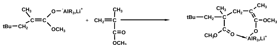
Scheme 1.6 : Aluminum ate complex and its penultimate co-ordination
