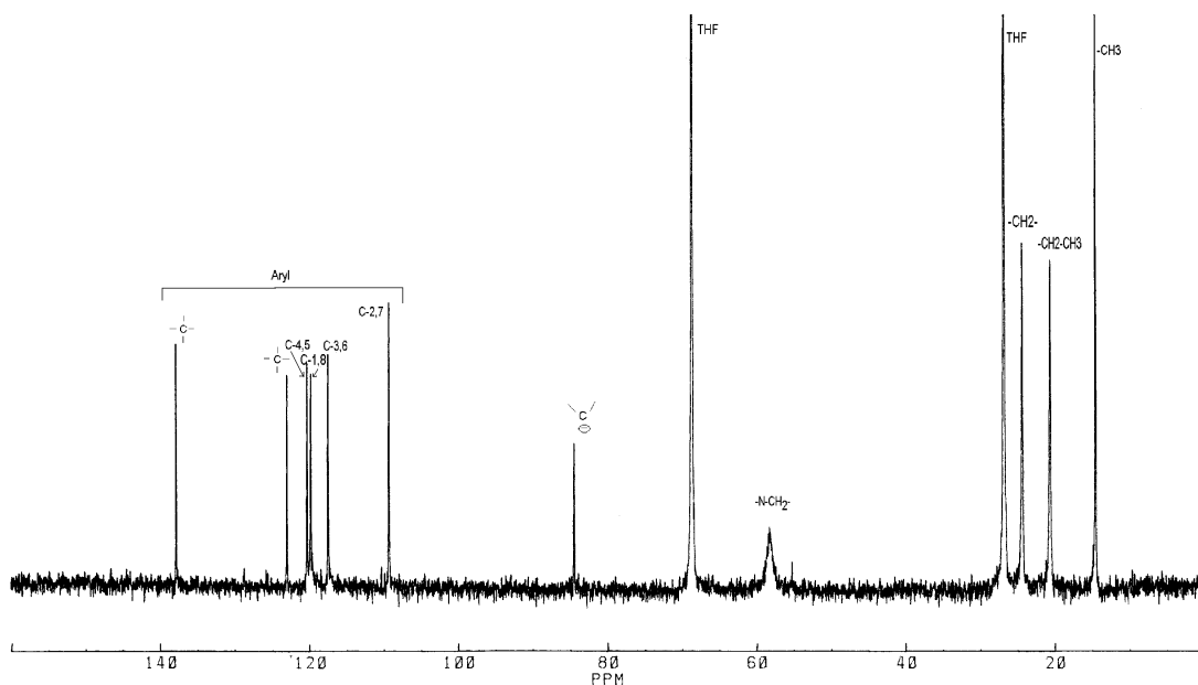
Fig. 7.3: 13 C NMR of tetrabutylammoniumfluorene salt, 2a in THF prepared by deprotonation method.
