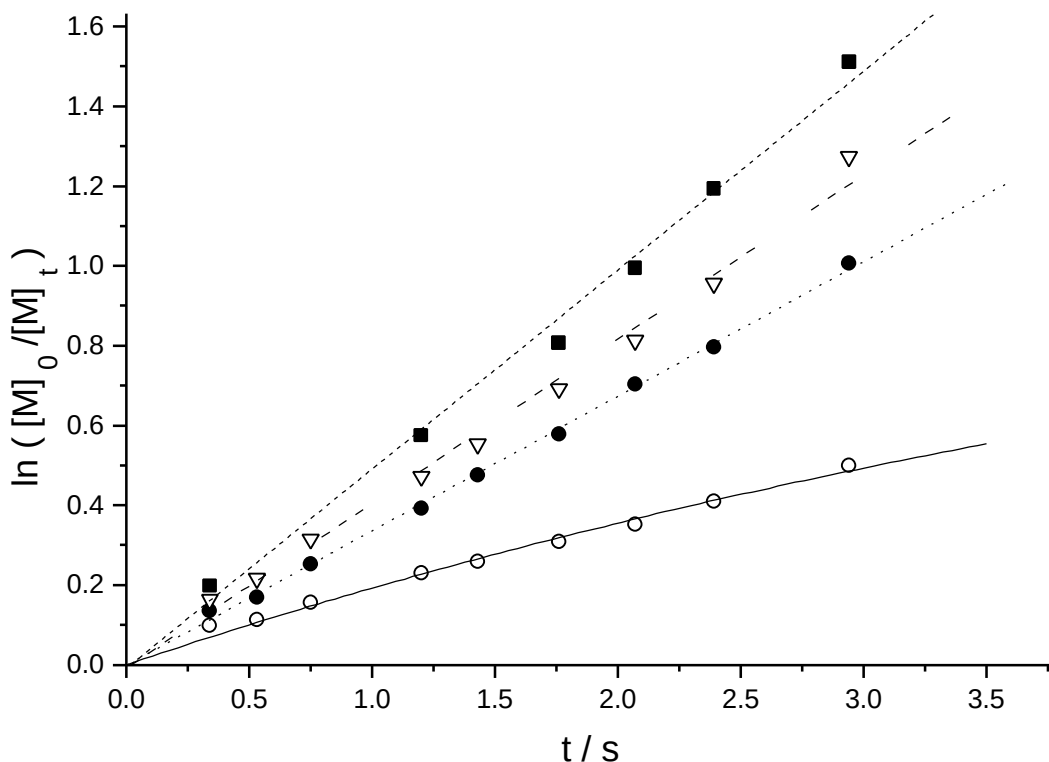
Fig. 5.7: First-order time-conversion plots of the MMA polymerization in THF
