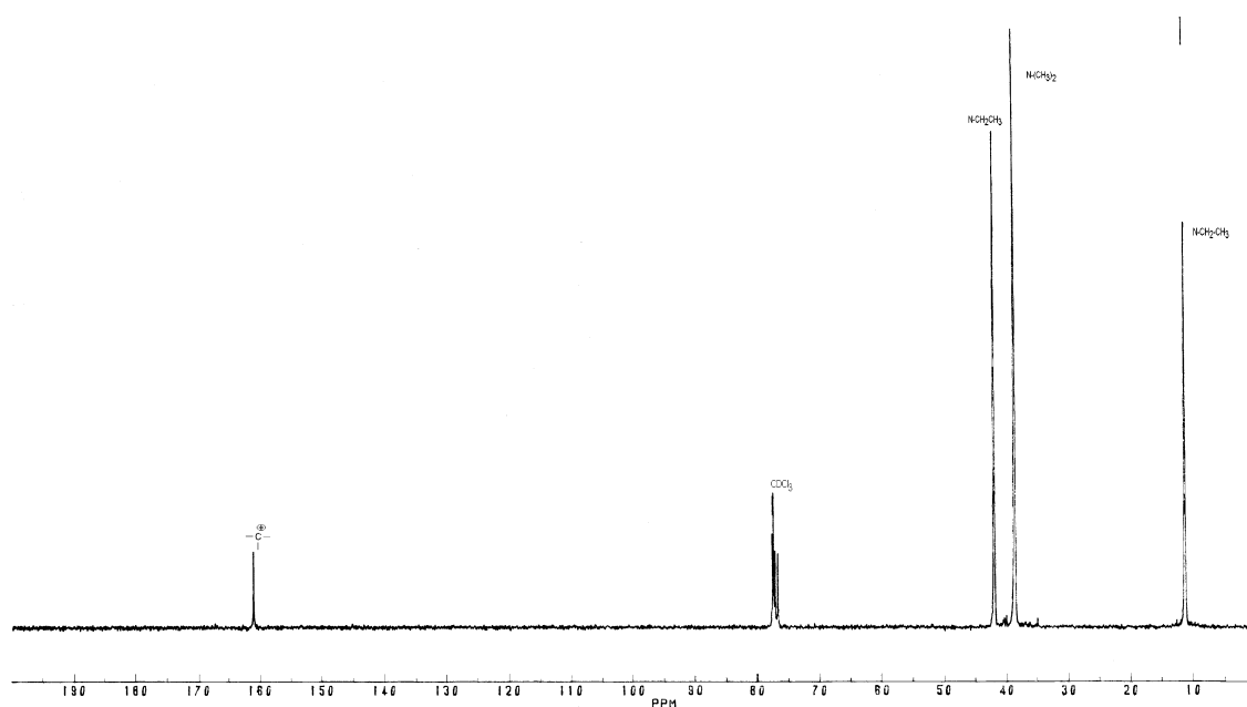
Fig. 7.1: 13 C NMR of tetramethyldiethylquaternidinium chloride in CDCl 3 at 30°C.
