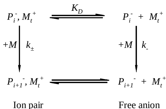
Scheme 1.4 : Equilibrium of ion pairs and free anions in anionic polymerization
