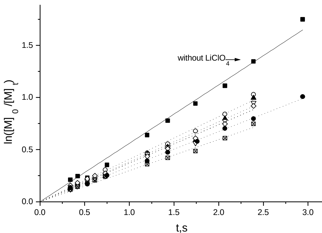
Fig. 5.12: First-order time-conversion plots of MMA polymerization in THF in presence of various concentration of \text{LiClO}_4 at -20^\circ\text{C} . r = [\text{LiClO}_4]_0/[\text{DPHLi}]_0 ; (■) r = 0 , (○) r = 0.3 , (▲) r = 0.6 , (Δ) r = 1 , (◇) r = 3 , (⊠) r = 5 , and (●) r = 10 .
