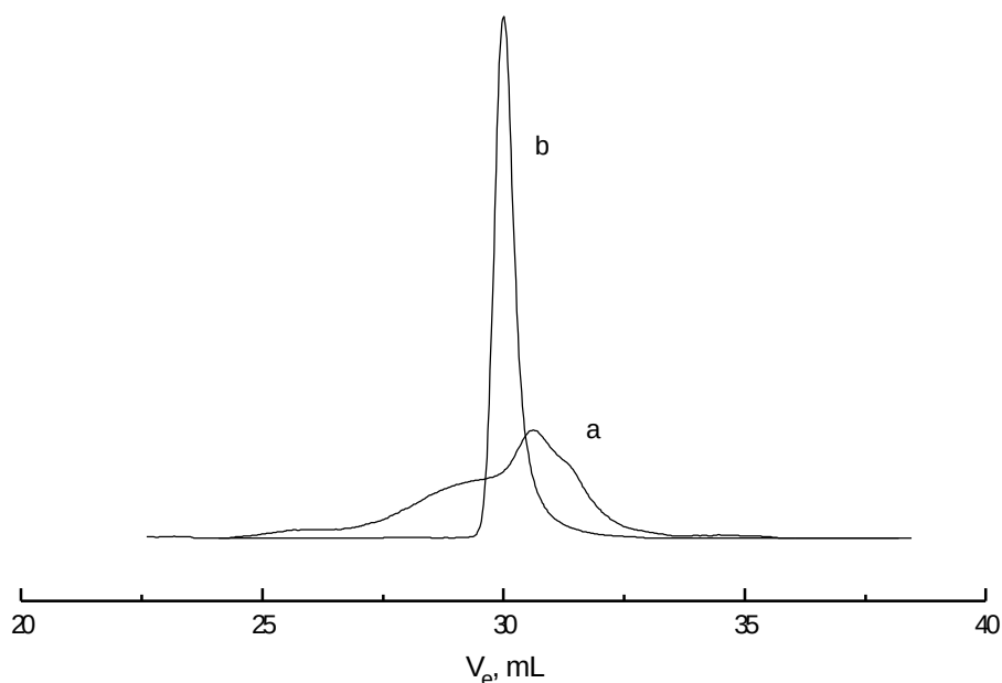
Fig. 5.3: SEC traces of PMMA synthesized in presence (b) and absence (a) of \text{LiClO}_4 in Toluene/THF (9:1, v/v) mixed solvent at -78^\circ\text{C} (run No. 12 and 15 in Table 5.5).
