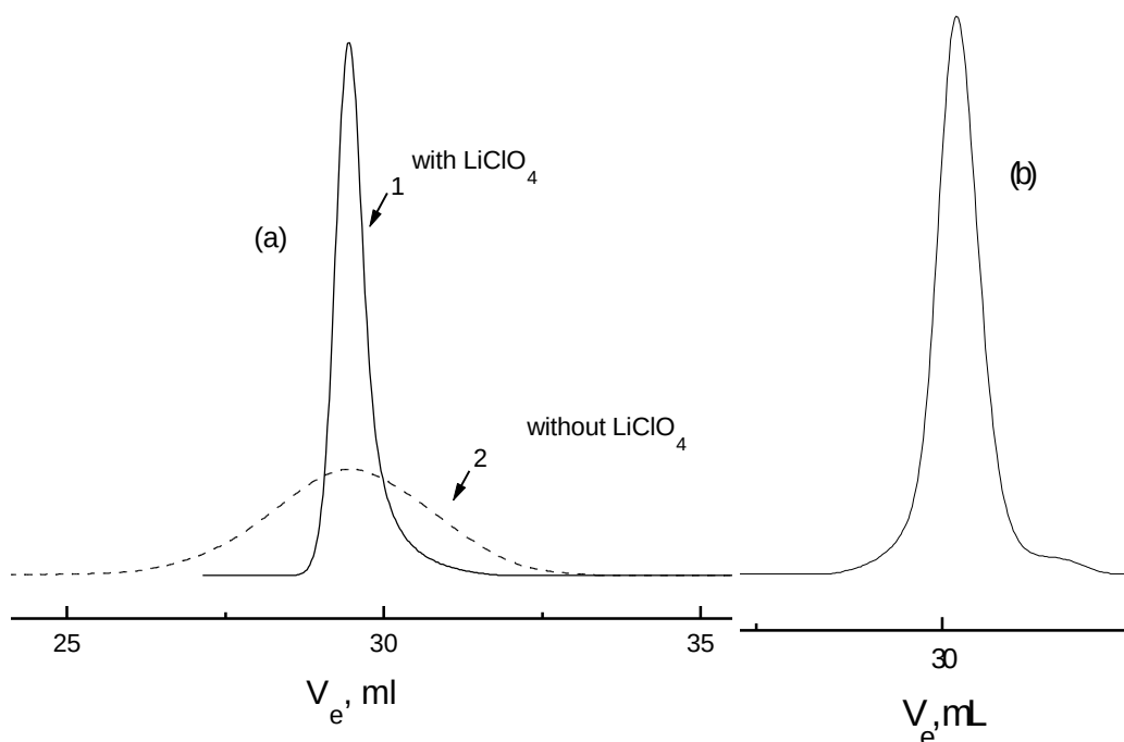
Fig. 5.2: Influence of \text{LiClO}_4 on the synthesis of PtBA in THF at -78\text{ }^\circ\text{C} : (a) 1. in the presence of \text{LiClO}_4 , M_{n,\text{SEC}} = 78,980 , M_w/M_n = 1.06 (run No.9 in Table 5.3), and 2. in the absence of \text{LiClO}_4 , M_{n,\text{SEC}} = 63,170 , M_w/M_n = 2.10 (run No.1 in Table 5.3), (b) SEC trace of Poly(tert-butylacrylate-b-methyl methacrylate) diblock copolymer prepared in the presence of \text{LiClO}_4 .
