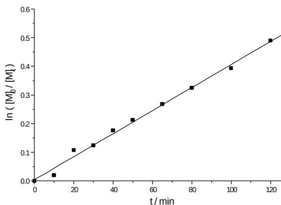
Fig.5.4: First-order time-conversion plot of MMA polymerization in Toluene/THF (9:1, v/v) mixed solvent in presence of LiClO_4 at -78^\circ C
