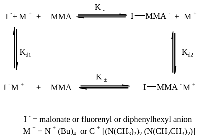
Scheme 7.2: Equilibrium addition of initiator to MMA and their ion-pairing effect
