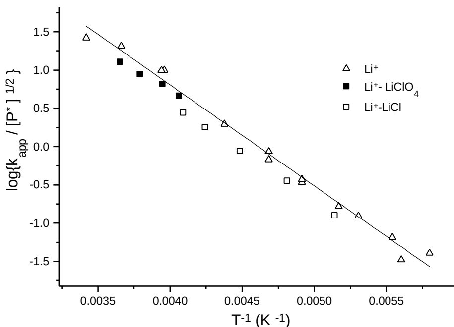
Fig. 5.17: The inverse square root dependence of rate constant, k_{app} at different
