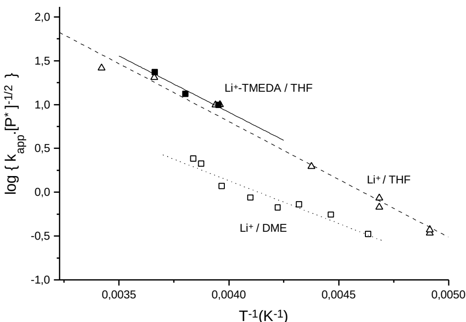
Fig. 4.10: The square root dependence of apparent rate constant, k_p on the active center concentration, [P^*] in anionic polymerization of MMA for TMEDA chelated Li^+ counterion ( r < 3 ) in THF and the reported rate constants in DME and THF solvent.
