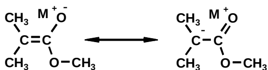
Scheme 6.3: Canonical forms of ester enolates
