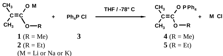
Scheme 6.4: Synthesis of tetraphenylphosphonium ester enolates
