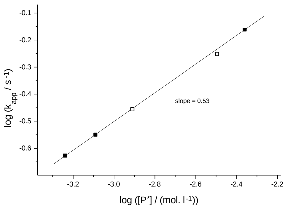
Fig. 4.4: Reaction order with respect to initiator concentration for the polymerization of MMA with TMEDA chelated \text{Li}^+ counterion in THF
