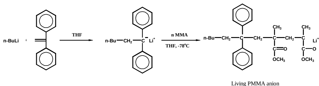
Scheme 1.2: Polymerization of MMA using 1,1'-diphenylhexyllithium as initiator
