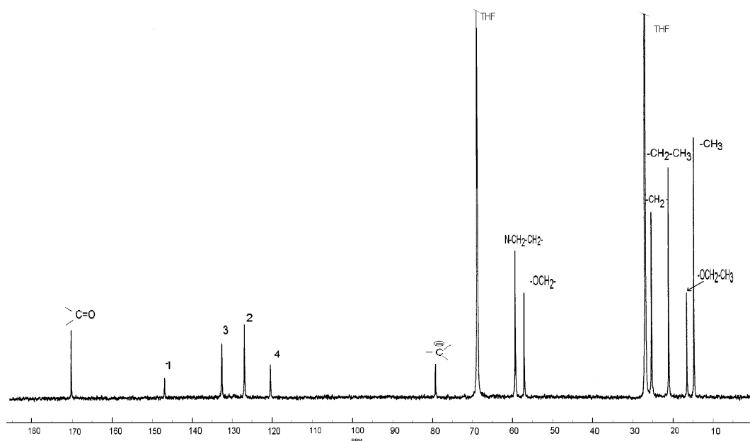
Fig 7.2: 13 C NMR of tetrabutylammonium diethylphenylmalonate, 2a in THF at 30°C. The initiator was prepared by deprotonation method.
