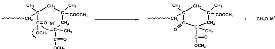
Scheme 1.1 : Secondary reactions in methyl methacrylate polymerization
