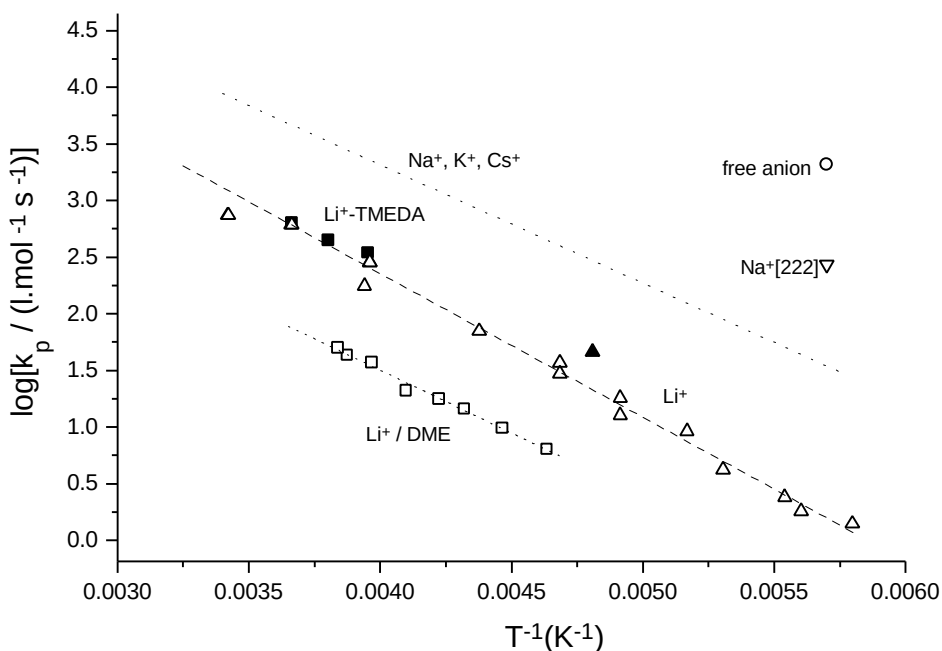
Fig. 4.9: Arrhenius plot of the propagation rate constants, k_p in the anionic polymerization of MMA for TMEDA chelated \text{Li}^+ counterion ( r < 3 ) in THF and the reported rate constant for other counterions and solvents (aggregation was not taken into account); (▲) k_+ rate constant at -65 \text{ }^\circ\text{C} .
