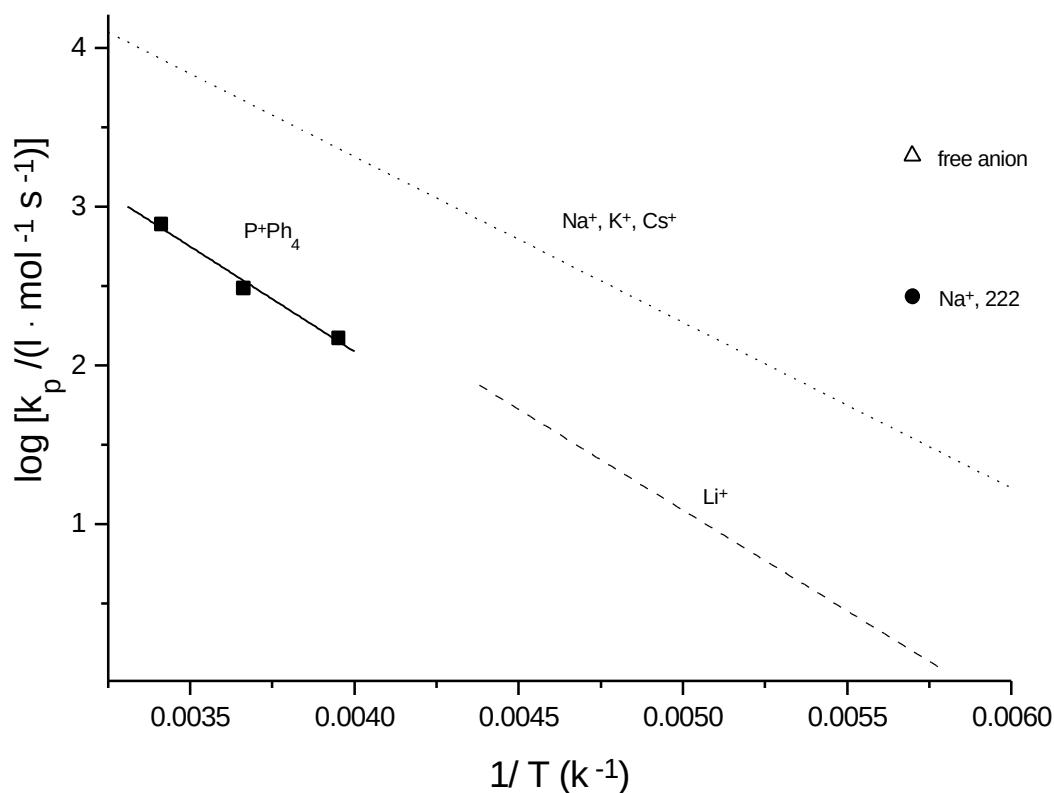
Fig. 6.10: Arrhenius plot of the overall propagation rate constants, k_p , in the anionic polymerization of MMA for PPh 4 counterion in THF and the reported rate constants of ion pairs for other counterions.
