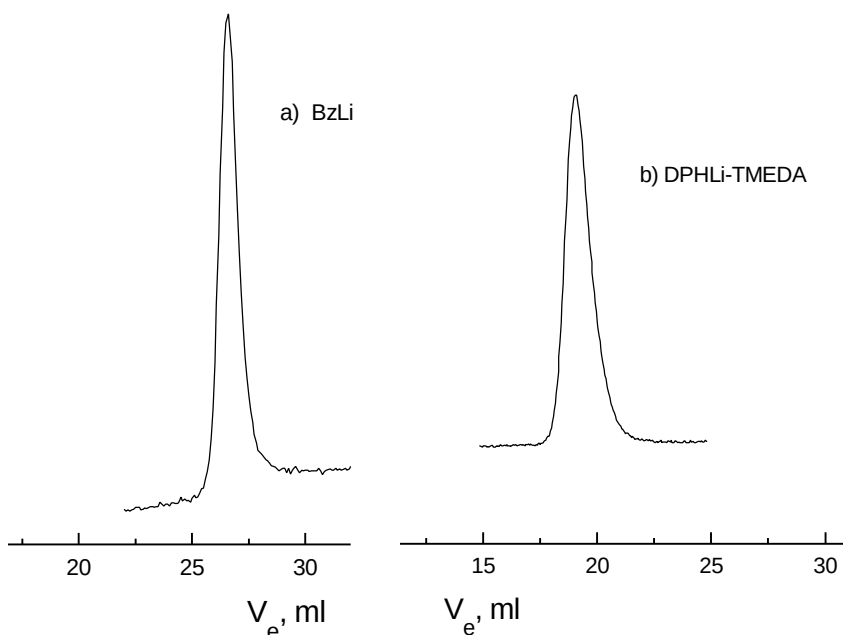
Fig. 4.1: SEC traces of PMMA prepared a) BzLi as initiator at -78\text{ }^{\circ}\text{C} and b) in presence of TMEDA using DPHLi at -40\text{ }^{\circ}\text{C} .
