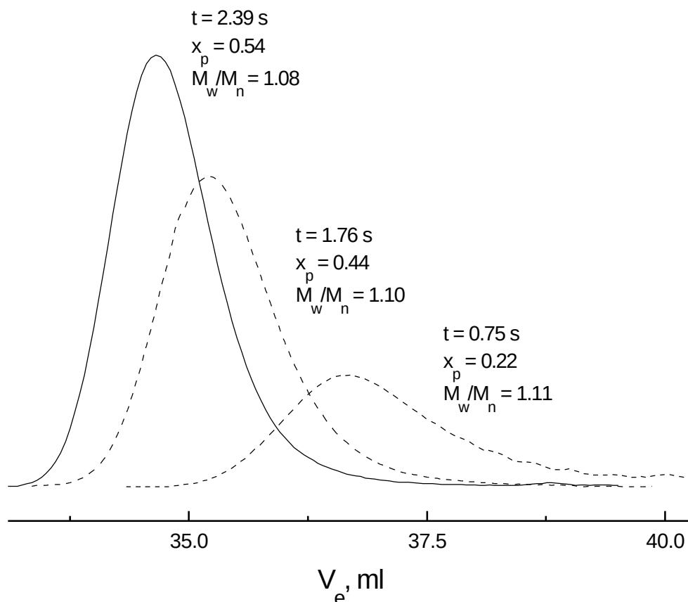
Fig. 5.11: SEC traces of PMMA at various time of polymerization in presence of \text{LiClO}_4 at -20^\circ\text{C} . (run no.3 in Table 5.8)
