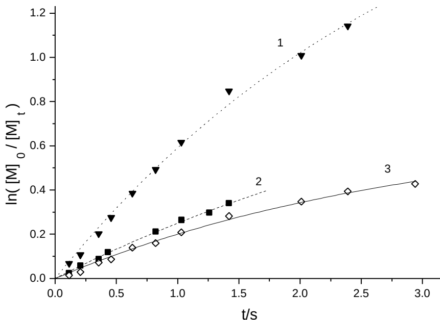
Fig.4.2: First-order time-conversion plots of the MMA polymerization in THF in presence of a 2-fold molar excess of TMEDA with respected to initiator concentration at -20 °C. [M]_0 = 0.23 mol/l, [I]_0 1) 5.9 \cdot 10^{-3} , 2) 1.4 \cdot 10^{-3} and 3) 0.8 \cdot 10^{-3} all in mol/l.
