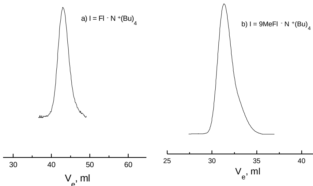
Fig. 7.5: GPC elugrams of PMMA synthesized in THF using initiator at 30 °C a) using 2a , M_{n,SEC} = 4140 , M_w/M_n = 1.32 and b) using 2b , M_{n,SEC} = 16,050 , M_w/M_n = 1.47 .
