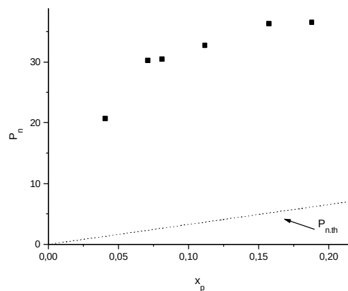
Fig. 6.12: Dependence of number-average degree of polymerization, P_n , on conversion x_p , using MiBPPH 4 as an initiator in THF at +20 °C
