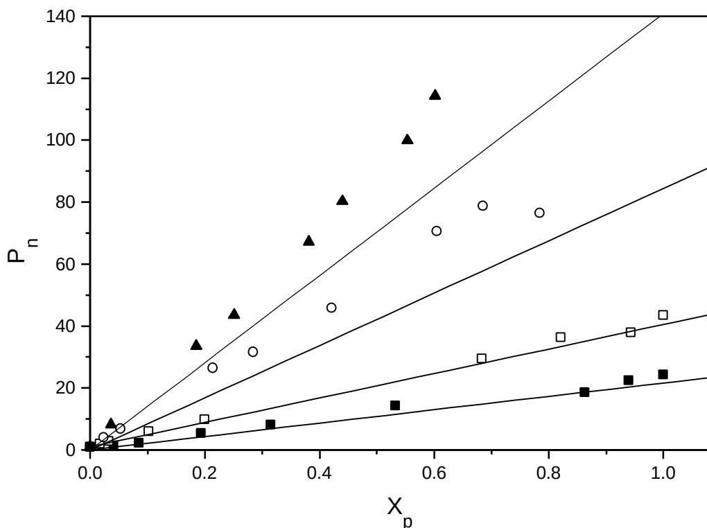
Fig. 6.3: Dependence of number-average degree of polymerization, P_n , on conversion, x_p , at 0 °C for the anionic polymerization of MMA in THF using PPh_4 as counterion. [M]_0 = 0.2 mol/L, [I]_0 ; (■) 9.95 \cdot 10^{-3} , (□) 5.3 \cdot 10^{-3} , (○) 2.37 \cdot 10^{-3} , and (▲) 1.42 \cdot 10^{-3} all in mol/L.
