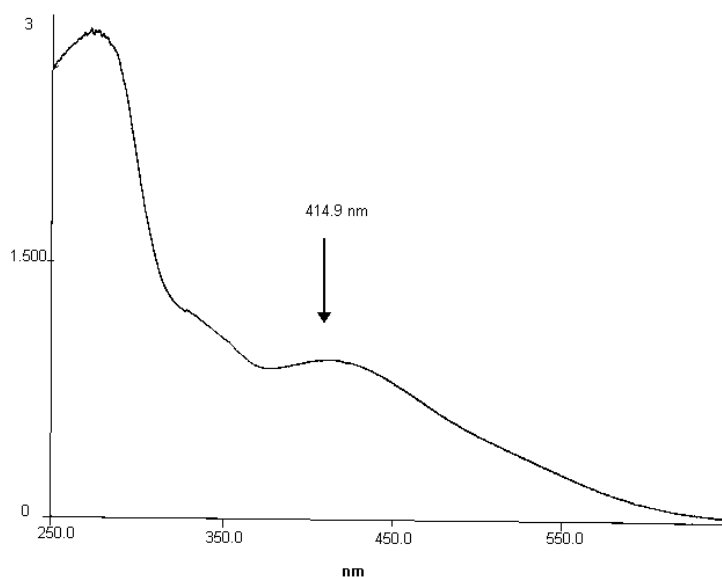
Fig. 6.13: UV/VIS absorption spectrum of 4 showing \lambda_{\text{max}} at \sim 415 nm
