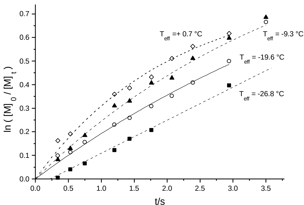
Fig. 5.15: First-order time-conversion plots at different temperatures. [\text{MMA}]_0 = 0.2 mol/L, [\text{I}]_0 = 1.4 \cdot 10^{-3} mol/L.
